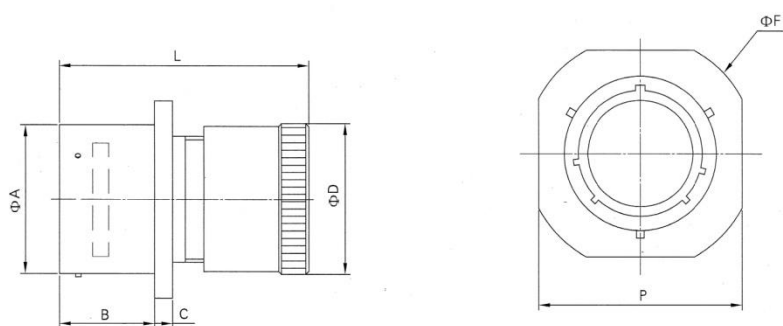
Cable connecting receptacle (MS3111E)
