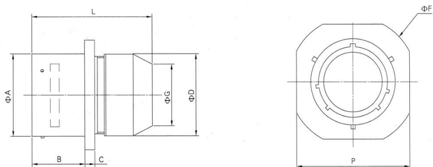
Cable connecting receptacle (MS3111P)
