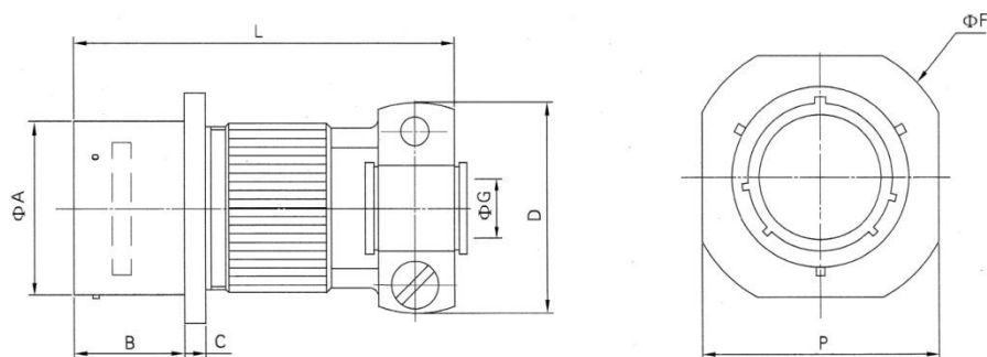
Cable connecting receptacle (MS3111F)
