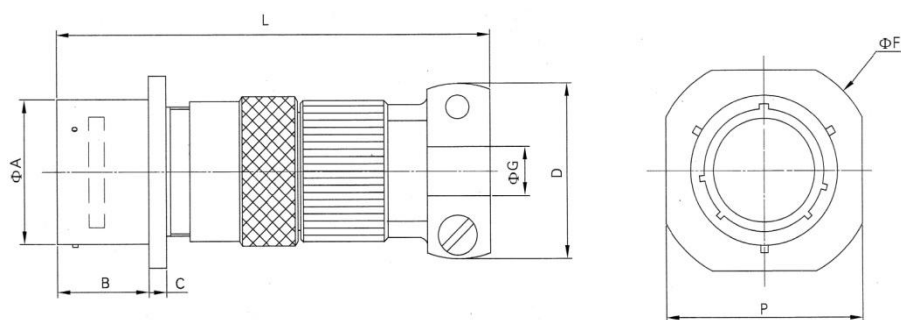
Cable connecting receptacle (MS3111J)
